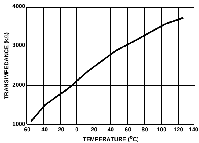
FIGURE 32. TRANSIMPEDANCE vs TEMPERATURE
