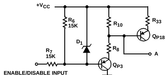
FIGURE 8. SIMPLIFIED SCHEMATIC OF ENABLE/DISABLE FUNCTION
