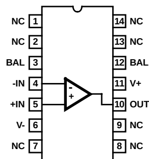
HA1-2541 (CERDIP) TOP VIEW
