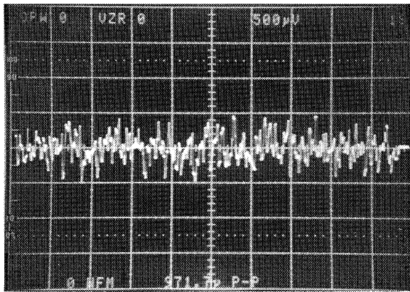
0.1Hz to 10Hz, Noise Voltage = 0.97 \mu V_{p.p} FIGURE 10. NOISE VOLTAGE ( A_V = 1000 )
