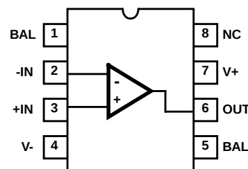
HA-2544 (CERDIP) HA-2544C (PDIP) TOP VIEW
