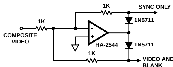
FIGURE 5. APPLICATION 2, COMPOSITE VIDEO SYNC SEPARATOR
