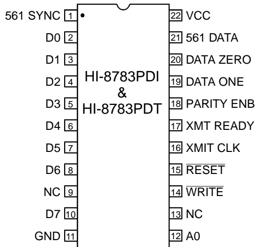
22 Pin DIP package
