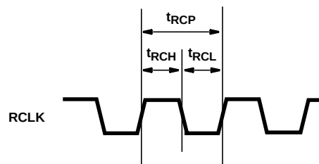
FIGURE 6. RCLK WAVEFORM
