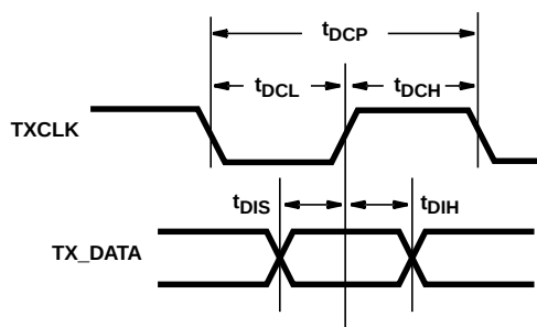
FIGURE 8. TRANSMIT DATA WAVEFORMS
