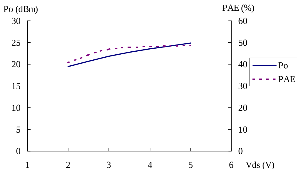
Output Power & Efficiency vs V_{ds} @ f=1.9\text{GHz} , I_{ds}=110\text{mA}
