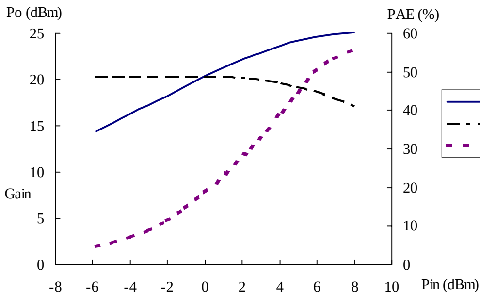
Output Power & Efficiency & Gain vs Input Power @ f=0.9\text{GHz} , V_{ds}=5\text{V}
