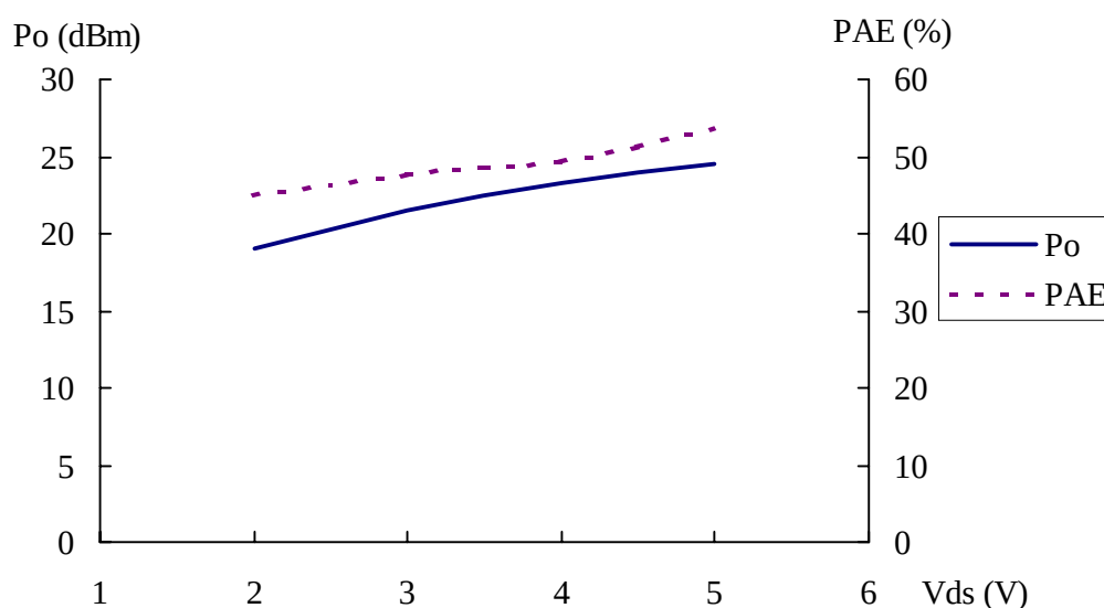
Output Power & Efficiency vs V_{ds} @ f=0.9\text{GHz} , I_{ds}=110\text{mA}
