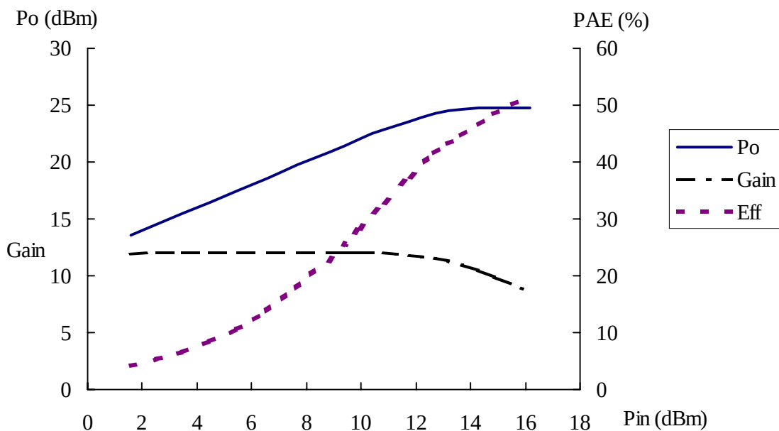
Output Power & Efficiency & Gain vs Input Power @ f=1.9\text{GHz} , V_{ds}=5\text{V}
