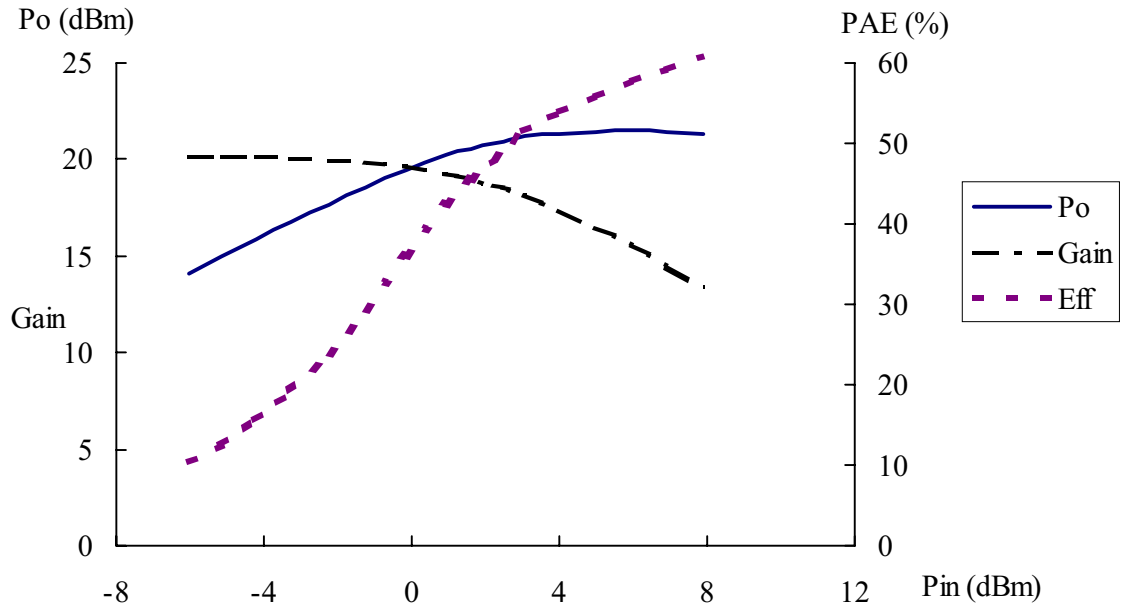
Output Power & Efficiency & Gain vs Input Power @ f=0.9\text{GHz} , V_{ds}=5\text{V}
