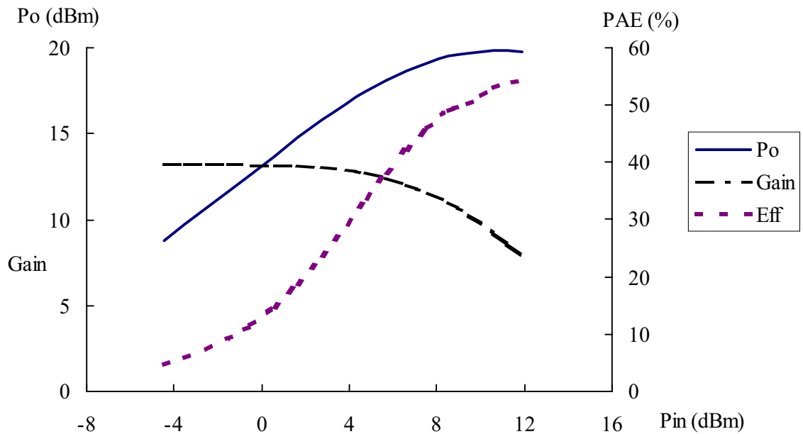
Output Power & Efficiency & Gain vs Input Power @ f=1.9\text{GHz} , V_{ds}=3\text{V}
