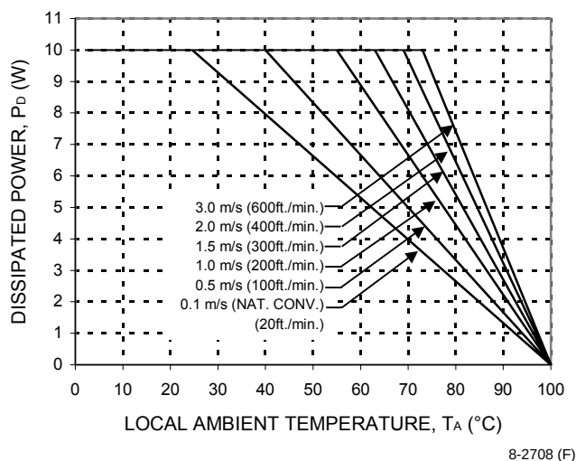
Figure 34. Power Derating vs. Local Ambient Temperature and Air Velocity; Best Orientation
