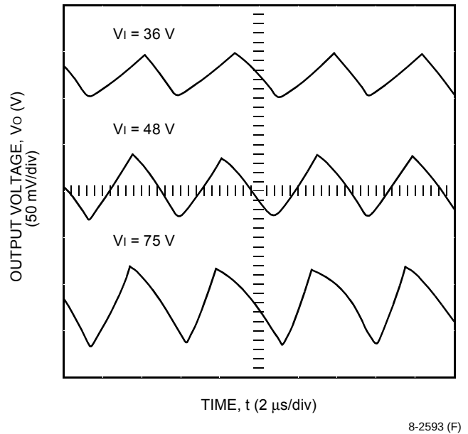
Figure 7. Typical HW050FG1 Output Ripple Voltage 3.3 V Output at Room Temperature and I_o = I_{o, \text{max}} , Different Input Voltage
