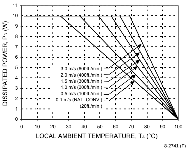
Figure 35. Power Derating vs. Local Ambient Temperature and Air Velocity; Worst Orientation
