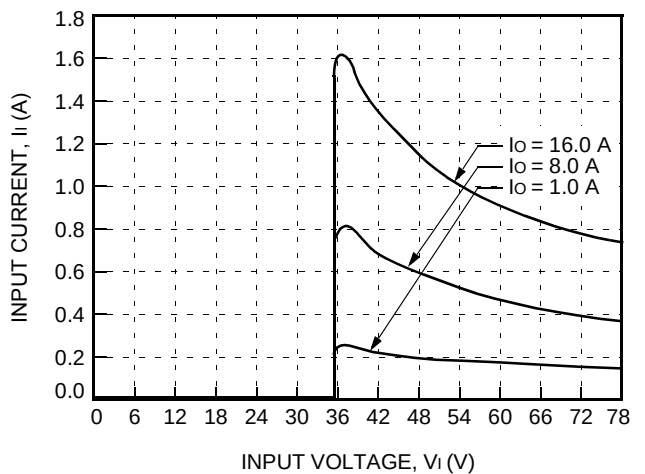
Figure 2. Typical HW050FG1 Input Characteristics at Room Temperature
