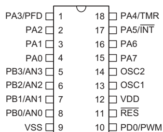
HT46C47 – 18 DIP-A/SOP-A
