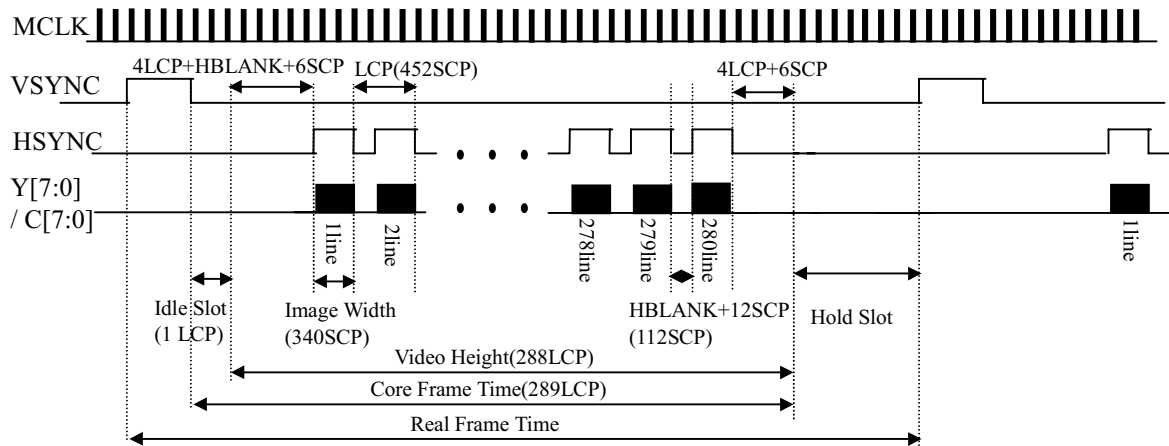
Figure 2. CIF Timing when Programmable Window is enabled
