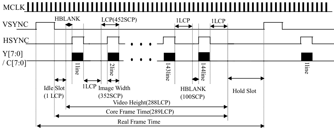
Figure 3. Sub-Sample CIF Timing when Programmable Window is disabled
