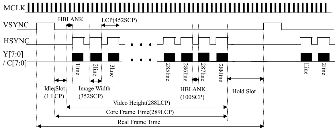
Figure 1. CIF Timing when Programmable Window is disabled
