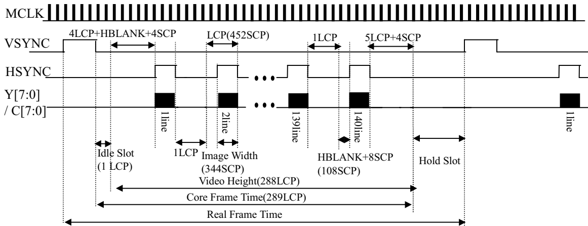
Figure 4. Sub-Sample CIF Timing when Programmable Window is enabled
