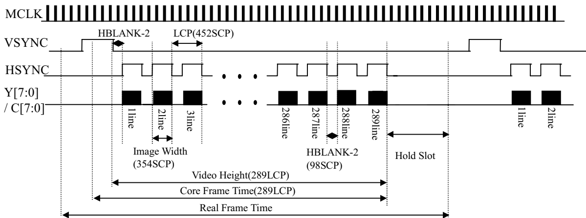
Figure 5. Bayer Output Timing
