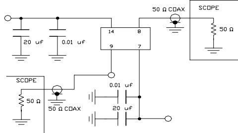
TEST CIRCUIT
