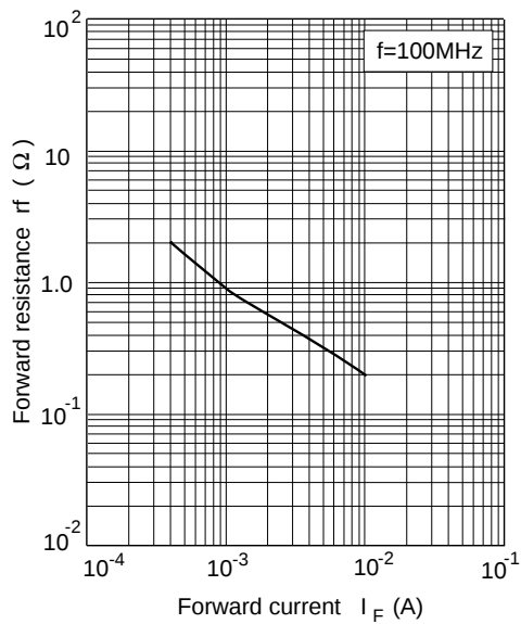
Fig.3 Forward resistance Vs. Forward current
