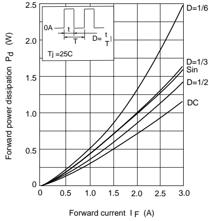
Fig.4 Forward power dissipation Vs. Forward current
