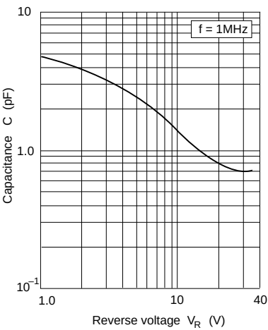
Fig.2 Capacitance Vs. Reverse voltage
