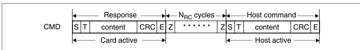
Timing Response End to Next CMD Start (Data Transfer Mode)
