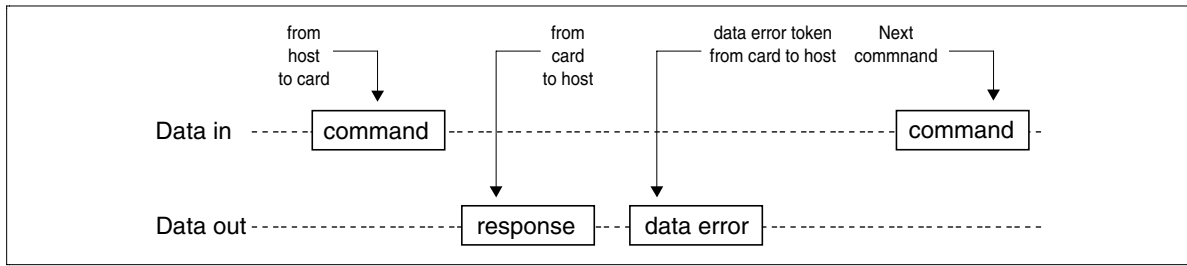
Read Operation-Data Error
