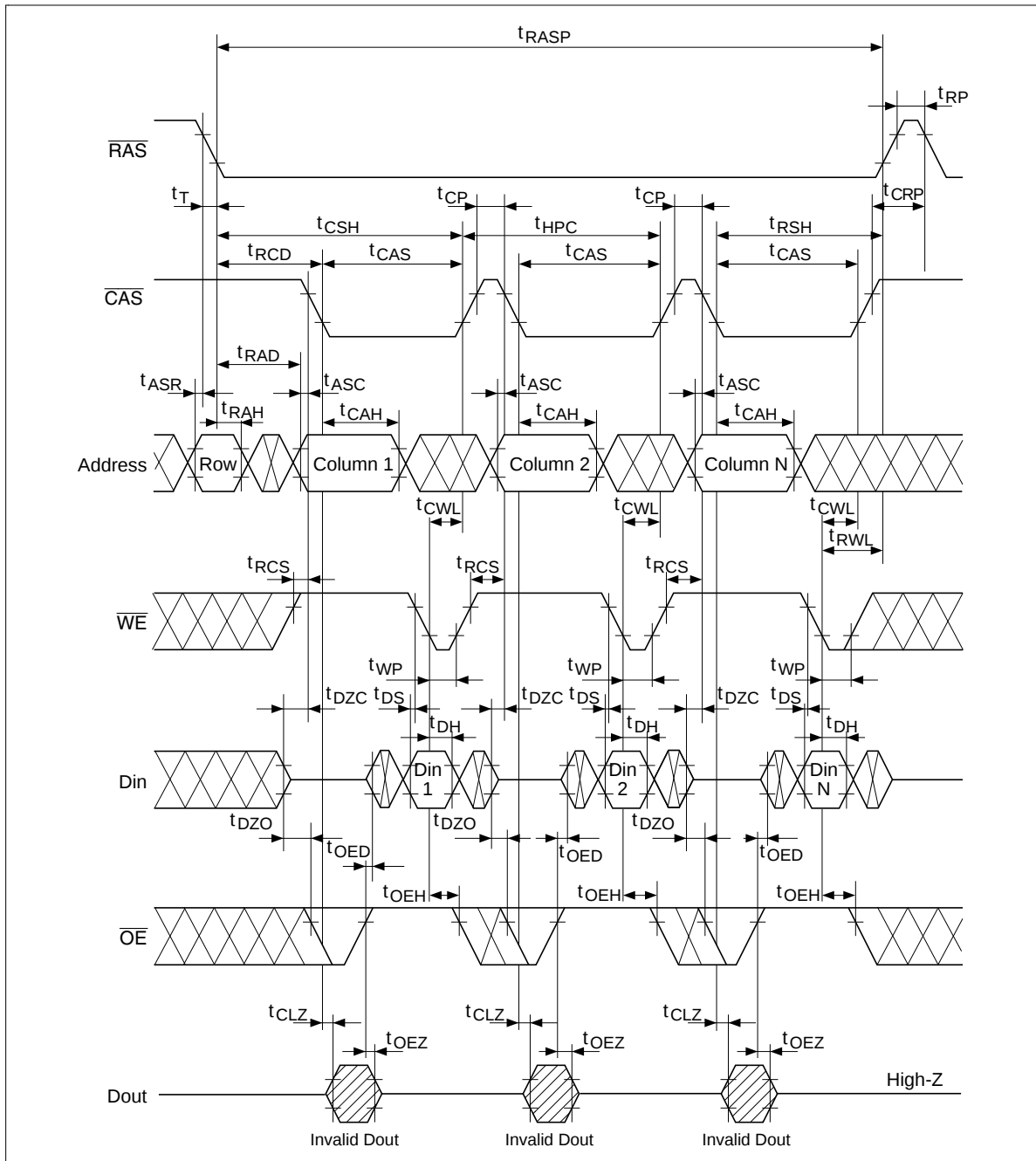
EDO Page Mode Read-Modify-Write Cycle *18
