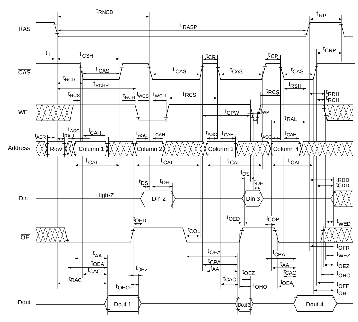
Self Refresh Cycle (L-version) *21, 22, 23, 24
