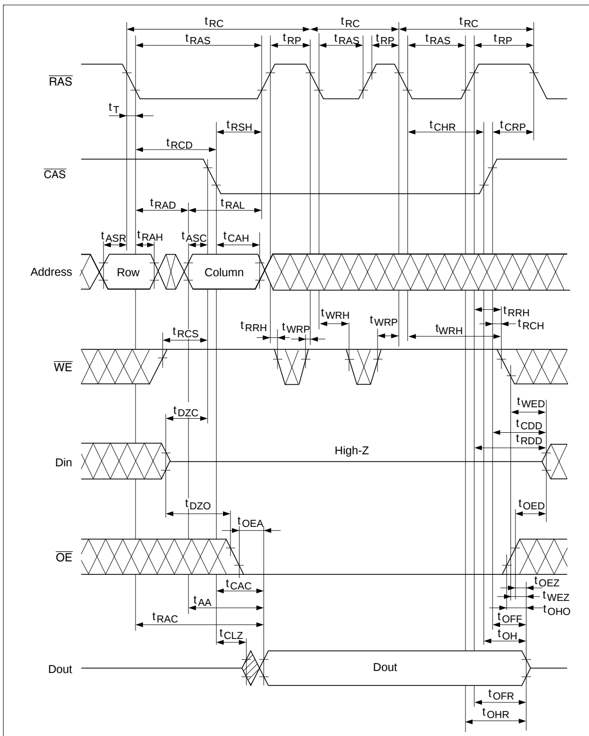
EDO Page Mode Read Cycle
