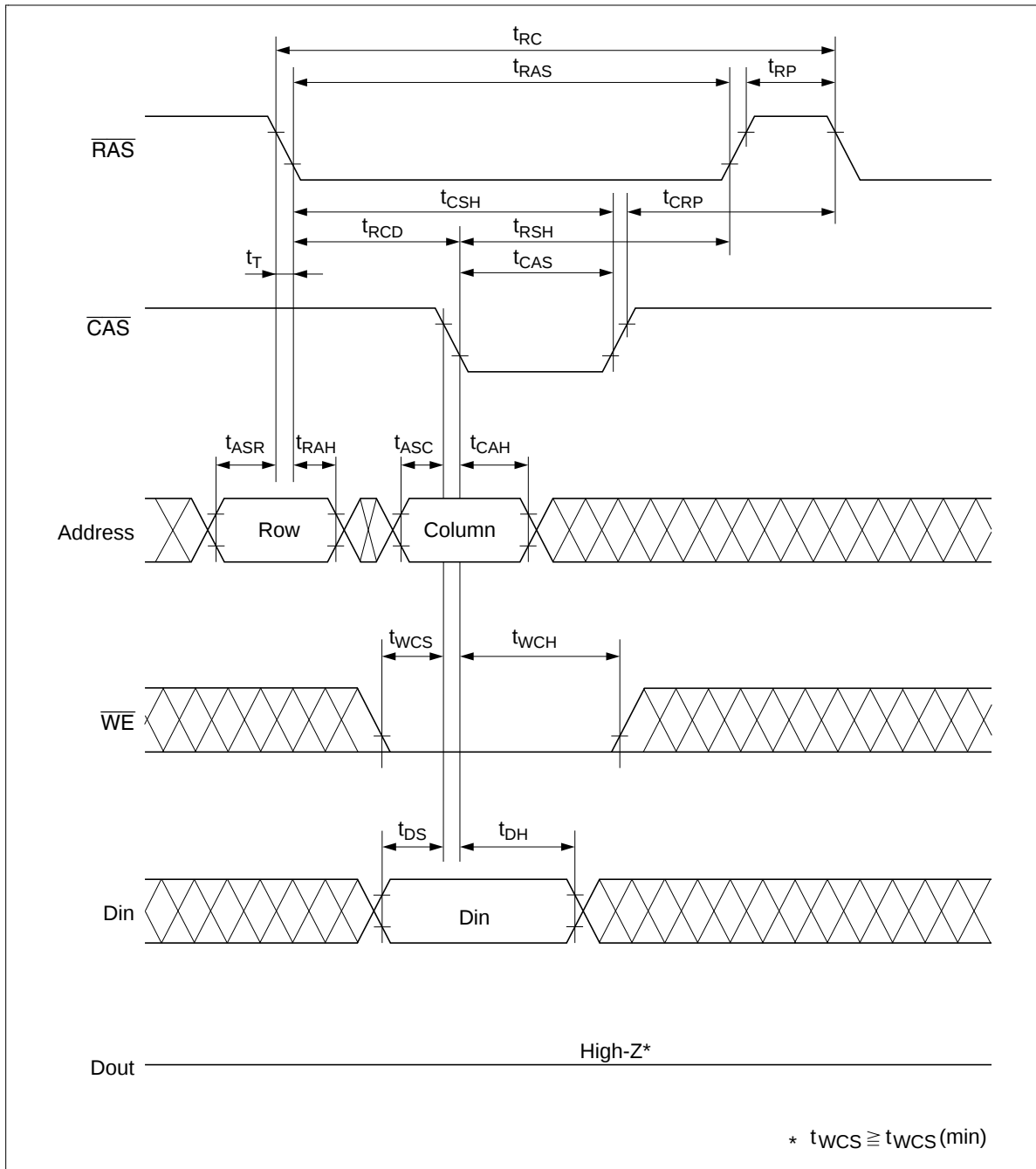
Delayed Write Cycle *18
