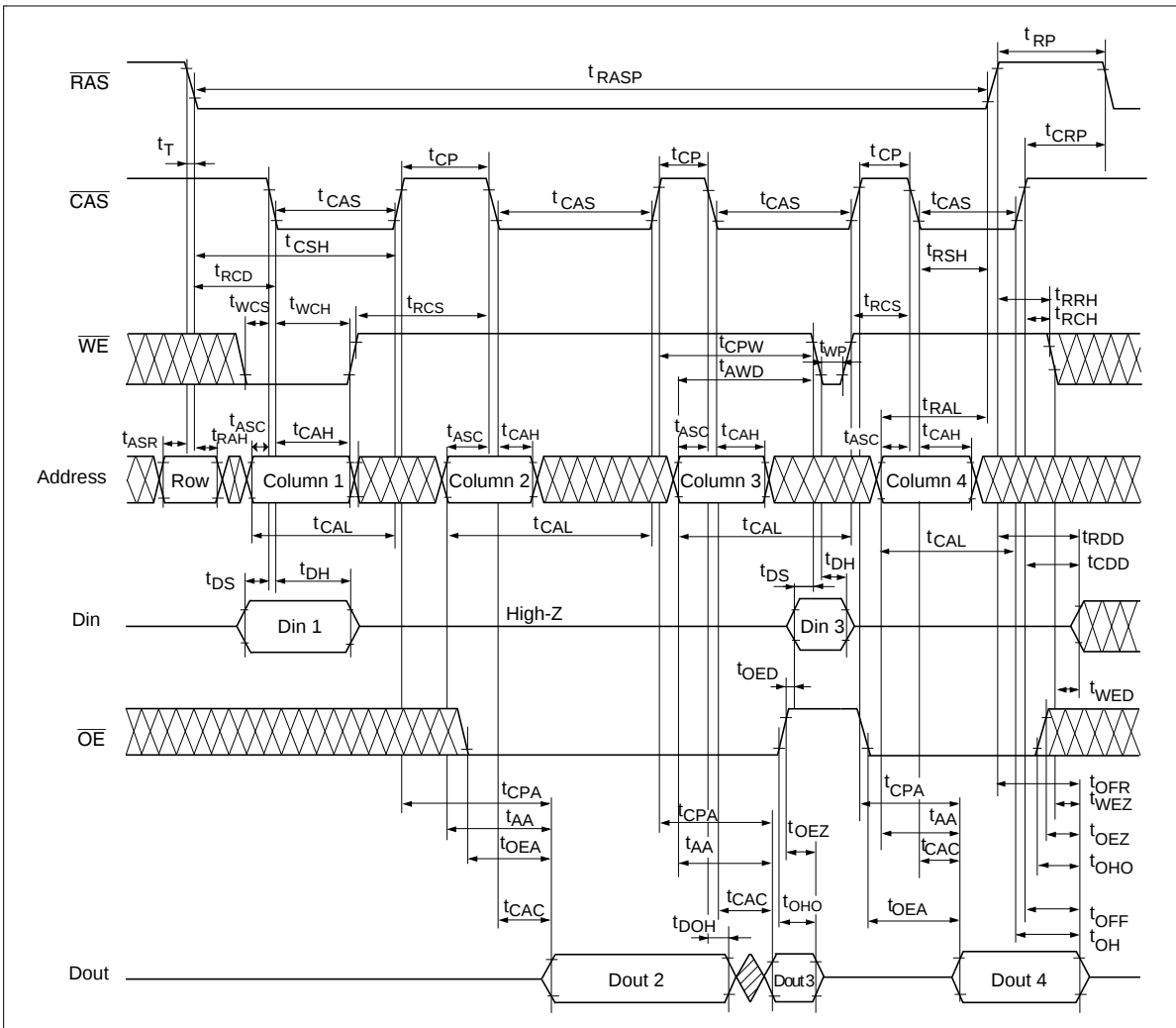
EDO Page Mode Mix Cycle (2)
