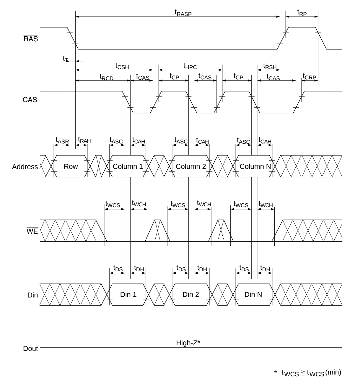
EDO Page Mode Delayed Write Cycle *18
