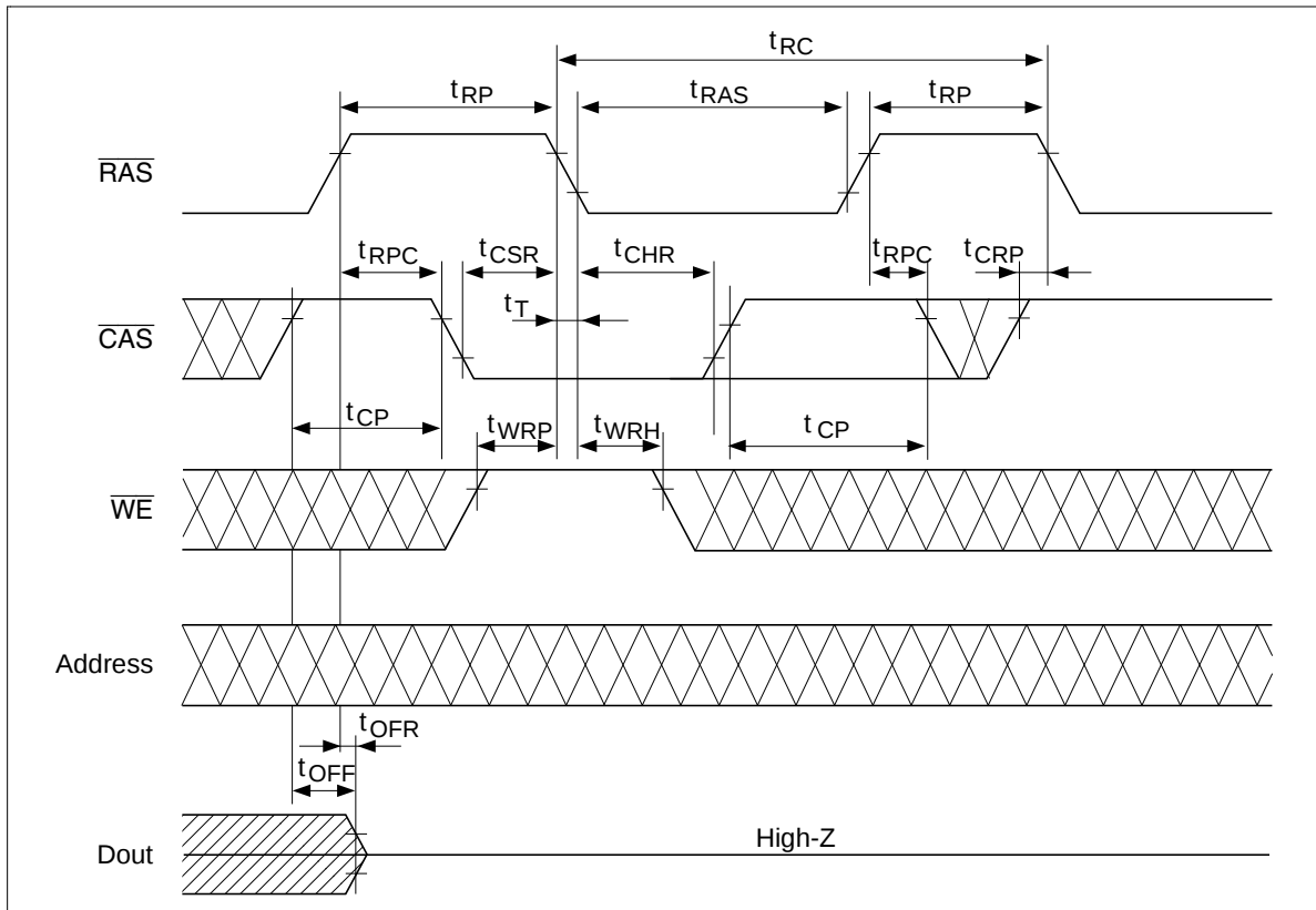
Hidden Refresh Cycle
