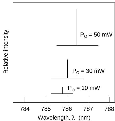
Lasing Spectrum
