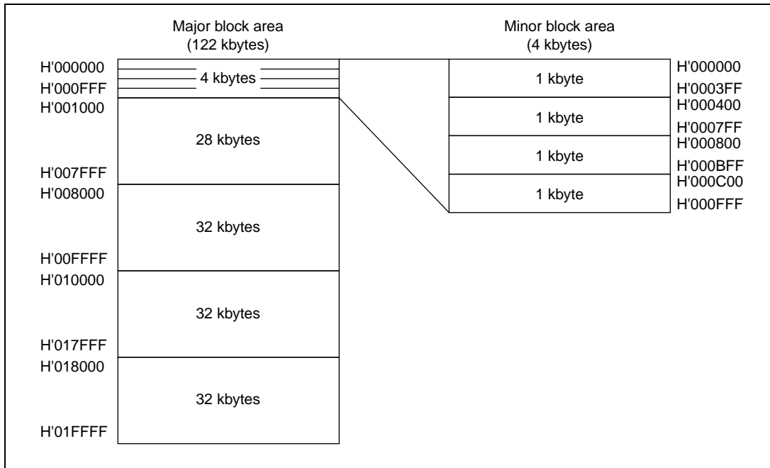
Figure 1.4 H8/3067F/62F Internal Flash Memory Block Divisions
