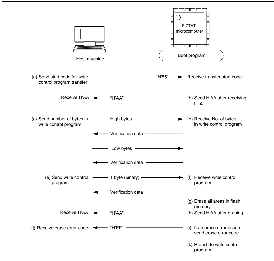
Figure 2.16 Write Control Program Transfer
