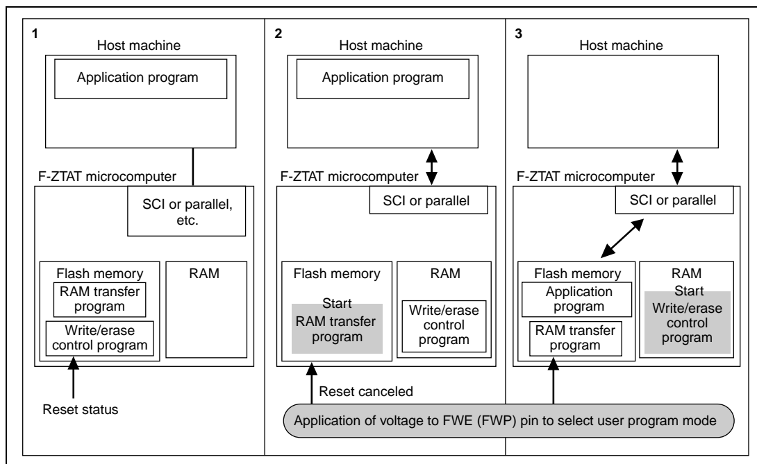
Figure 1.2 Overview of User Program Mode
