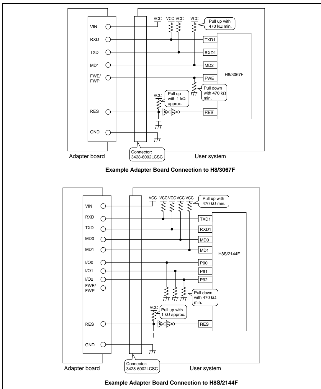
Figure 2.10 Example Adapter Board and F-ZTAT Microcomputer Connections (2)
