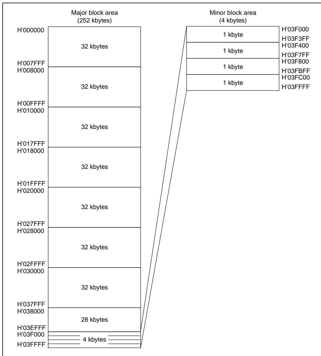
Figure 1.8 SH7044F/45F Internal Flash Memory Block Divisions
