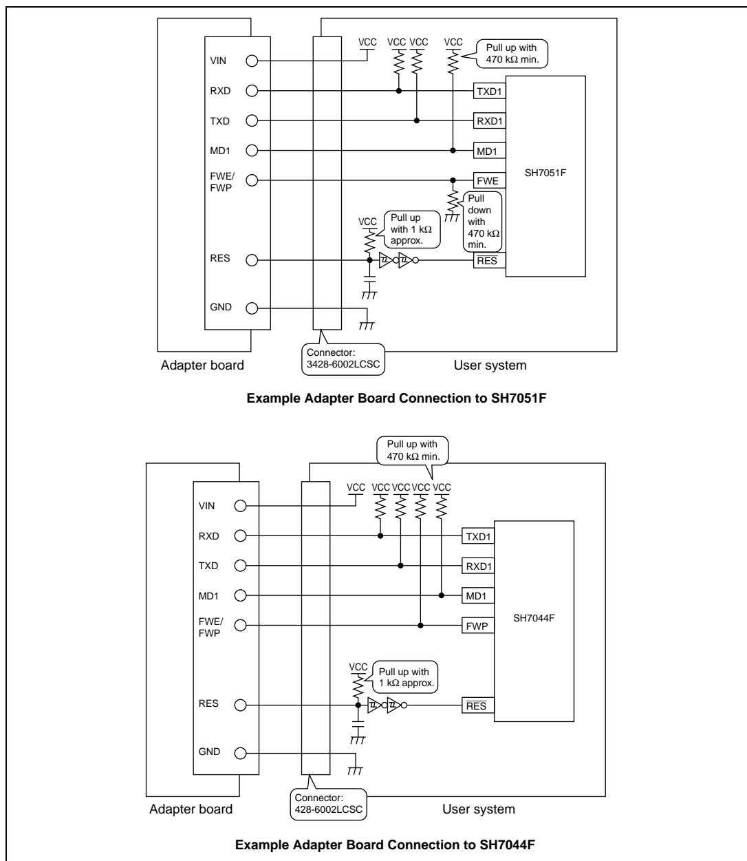
Figure 2.10 Example Adapter Board and F-ZTAT Microcomputer Connections (1)
