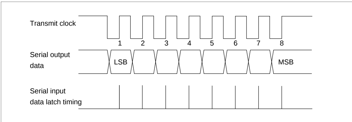
Figure 66 Serial Interface Output Timing
