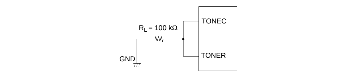
Figure 90 Distortion and \text{dB}_{\text{CR}} Load Circuit
