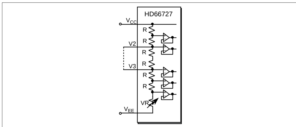
Figure 16 Contrast Adjuster
