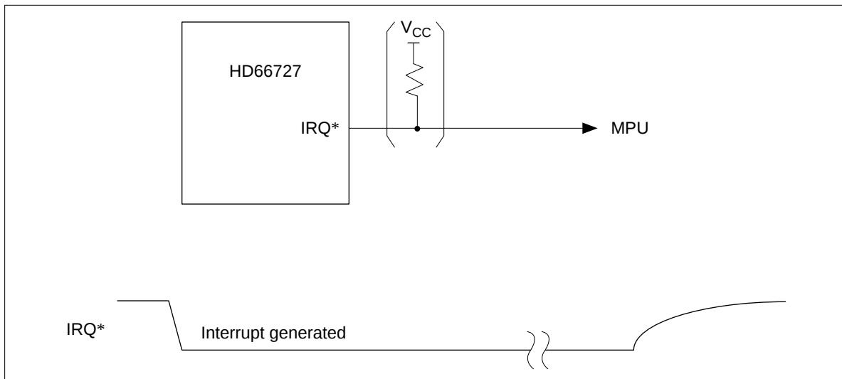
Figure 29 Interrupt Generation
