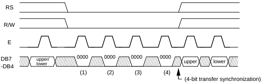
Figure 33 4-Bit Transfer Synchronization
