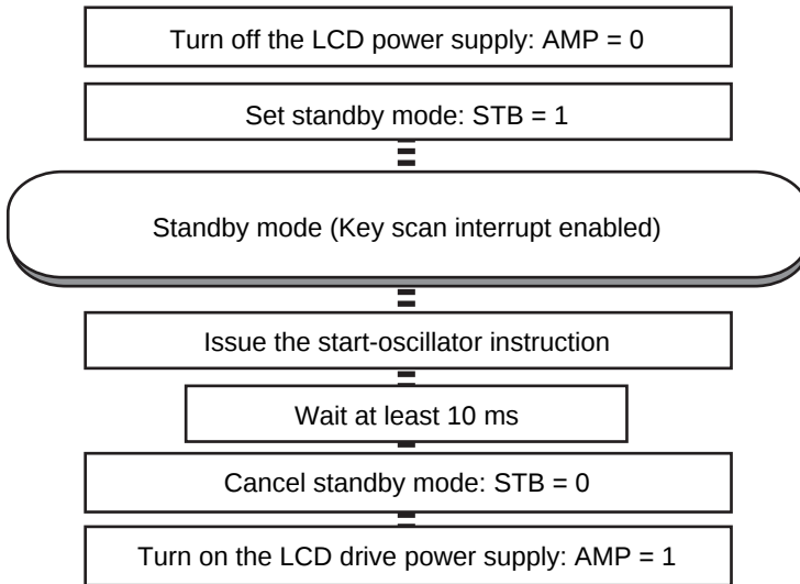
Figure 58 Procedure for Setting and Canceling Standby Mode
