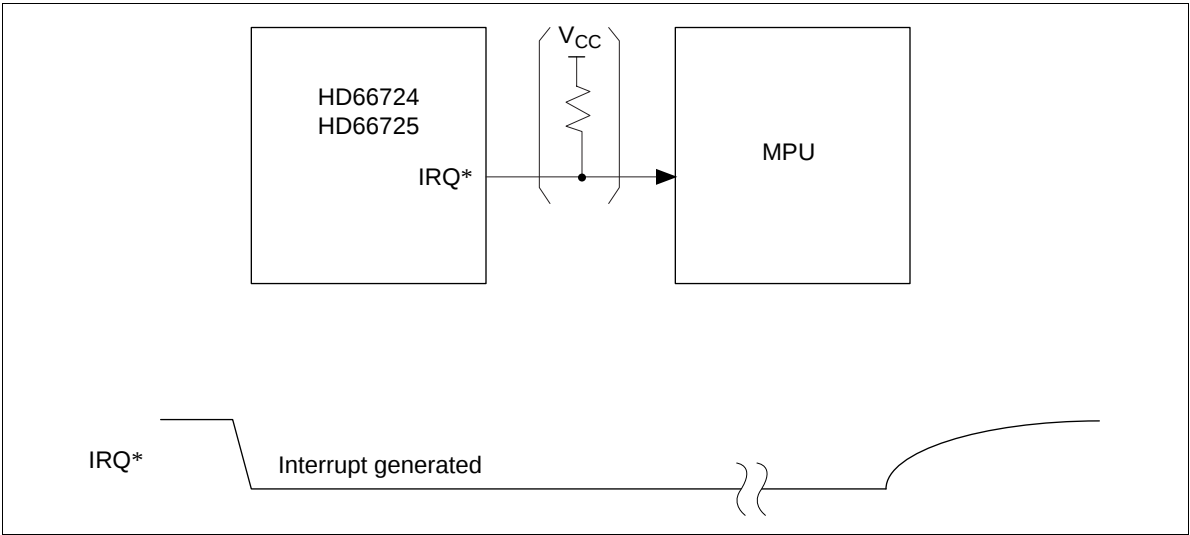
Figure 30 Interrupt Generation
