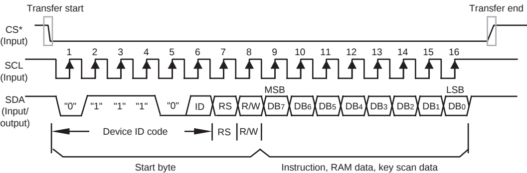
b) Consecutive Data-Transfer Timing through Clock-Synchronized Serial Bus Interface
