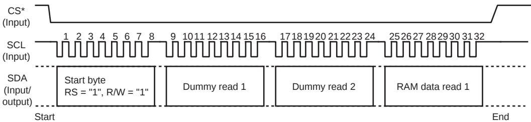
c) RAM Data Read-Transfer Timing
