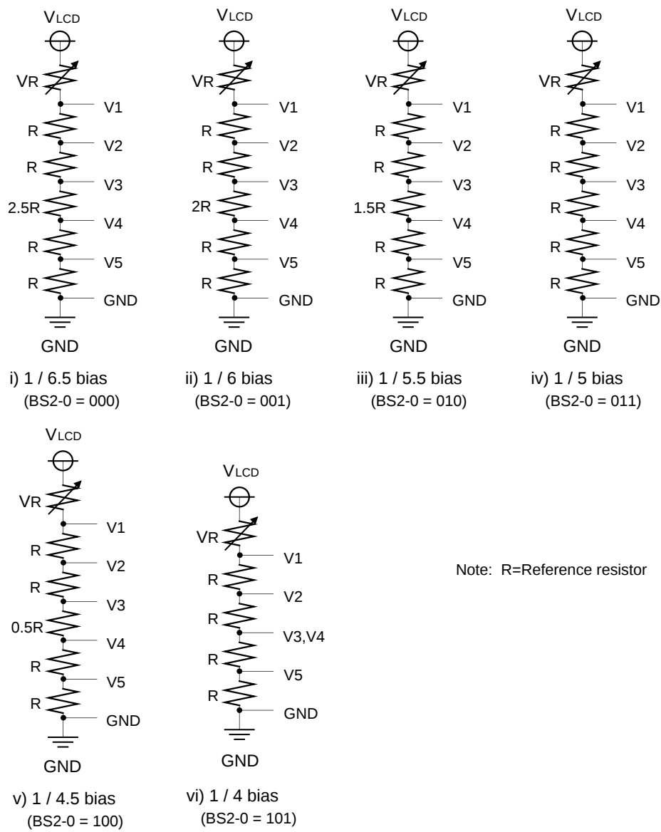
Figure 41 Liquid Crystal Display Drive Bias Circuit
