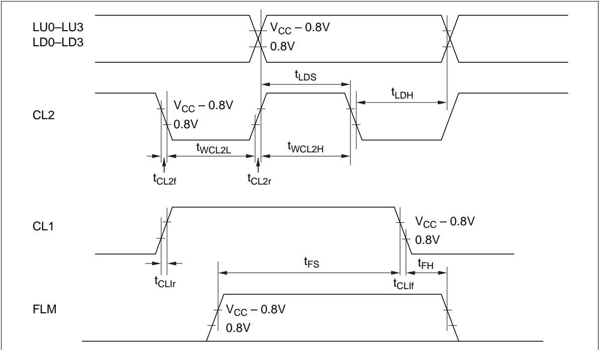
Figure 38 LCD Interface
