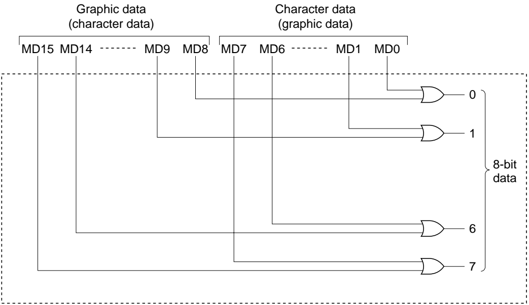
Figure 18 OR Function
