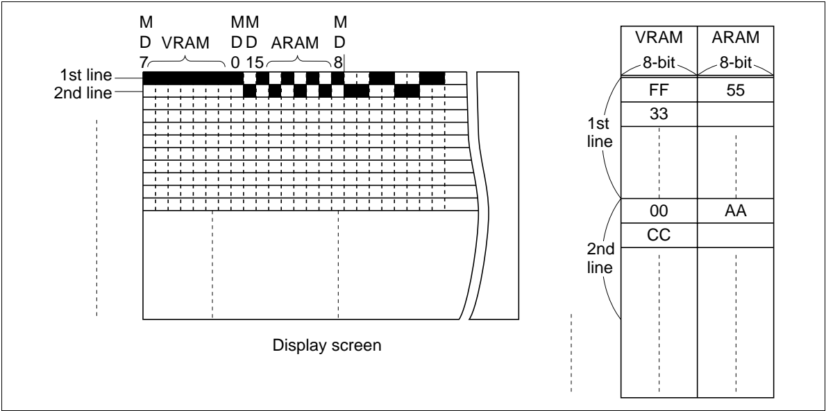
Figure 11 Relation between Graphic Screen and Memory Contents
