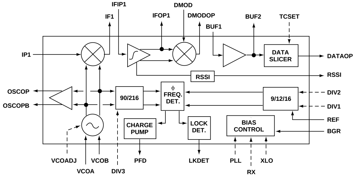
Figure 2. HPMX-5002 Detailed Block Diagram.
