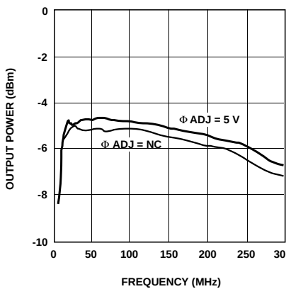
Figure 16. HPMX-2005 Output Power vs. Frequency and \Phi Adjust.
