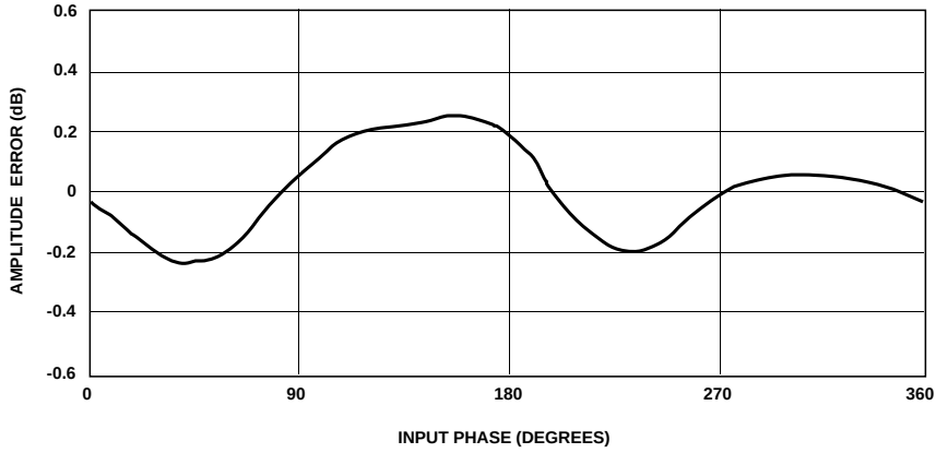
Figure 19. HPMX-2005 RMS Amplitude Error vs. Input Phase at 100 MHz.
