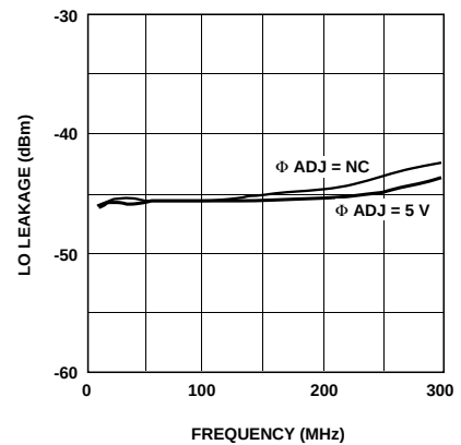
Figure 17. HPMX-2005 LO Leakage vs. Frequency and \Phi Adjust.
