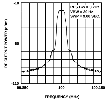
Figure 39. HPMX-2005 NADC Modulation Spectrum at 85^\circ\text{C} .
