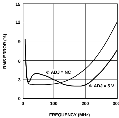
Figure 15. HPMX-2005 RMS Modulation Error vs. Frequency and \Phi Adjust.
