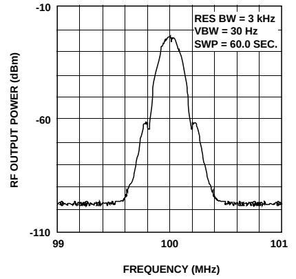
Figure 33. HPMX-2005 GSM Modulation Spectrum at 85^\circ\text{C} .
