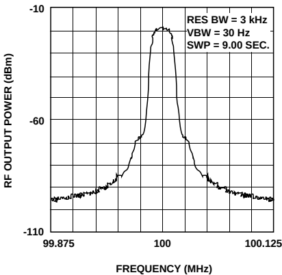
Figure 38. HPMX-2005 NADC Modulation Spectrum at 25^\circ\text{C} .
