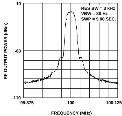
Figure 37. HPMX-2005 NADC Modulation Spectrum at -40^\circ\text{C} .
