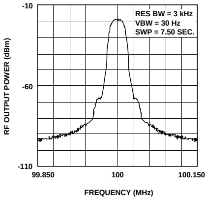
Figure 35. HPMX-2005 JDC Modulation Spectrum at 25^\circ\text{C} .
