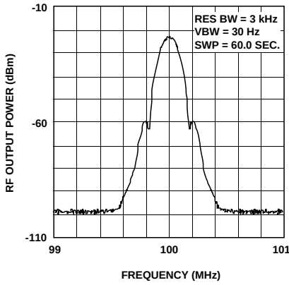
Figure 32. HPMX-2005 GSM Modulation Spectrum at 25^\circ\text{C} .
