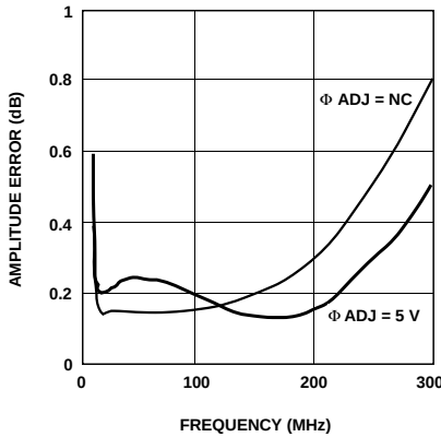
Figure 13. HPMX-2005 RMS Amplitude Error vs. Frequency and \Phi Adjust.
