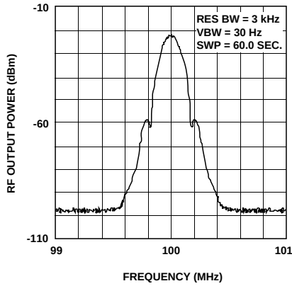
Figure 31. HPMX-2005 GSM Modulation Spectrum at -40^\circ\text{C} .
