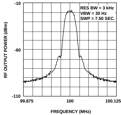
Figure 34. HPMX-2005 JDC Modulation Spectrum at -40^\circ\text{C} .
