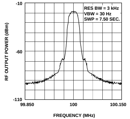
Figure 36. HPMX-2005 JDC Modulation Spectrum at 85^\circ\text{C} .
