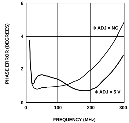
Figure 14. HPMX-2005 RMS Phase Error vs. Frequency and \Phi Adjust.
