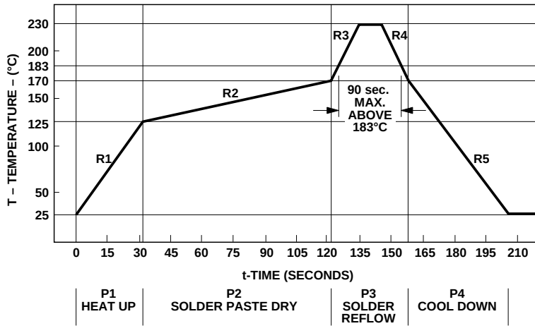
Figure 5. Reflow Profile.
