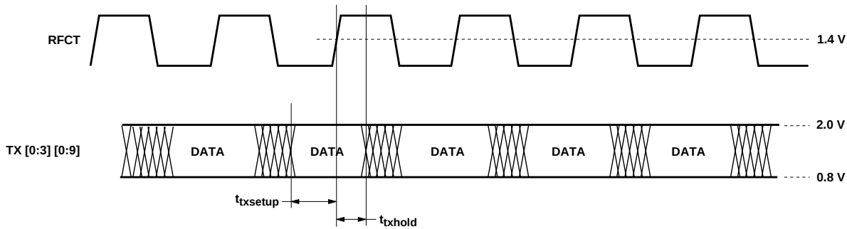
Figure 3. Transmitter section timing.
