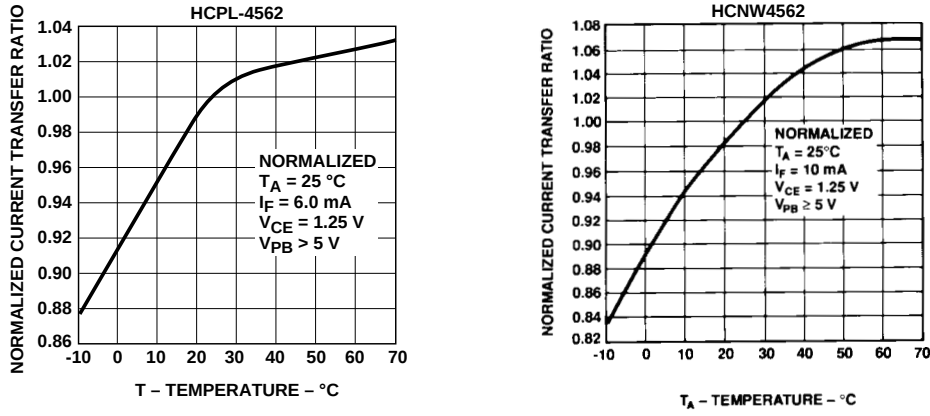
Figure 8. Current Transfer Ratio vs. Temperature.
