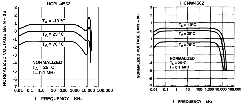
Figure 11. Normalized Voltage Gain vs. Frequency.
