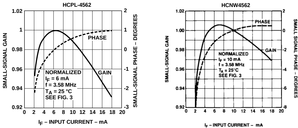
Figure 7. Small-Signal Response vs. Input Current.
