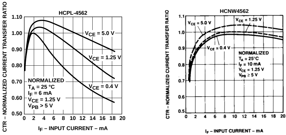
Figure 9. Current Transfer Ratio vs. Input Current.
