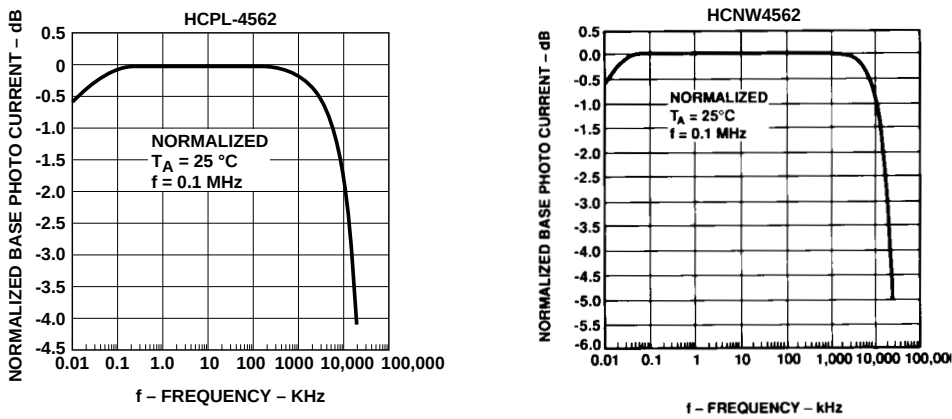
Figure 12. Normalized Base Photo Current vs. Frequency.
