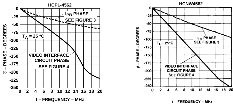
Figure 13. Phase vs. Frequency.
