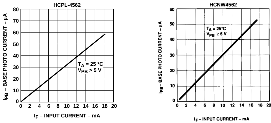
Figure 6. Base Photo Current vs. Input Current.
