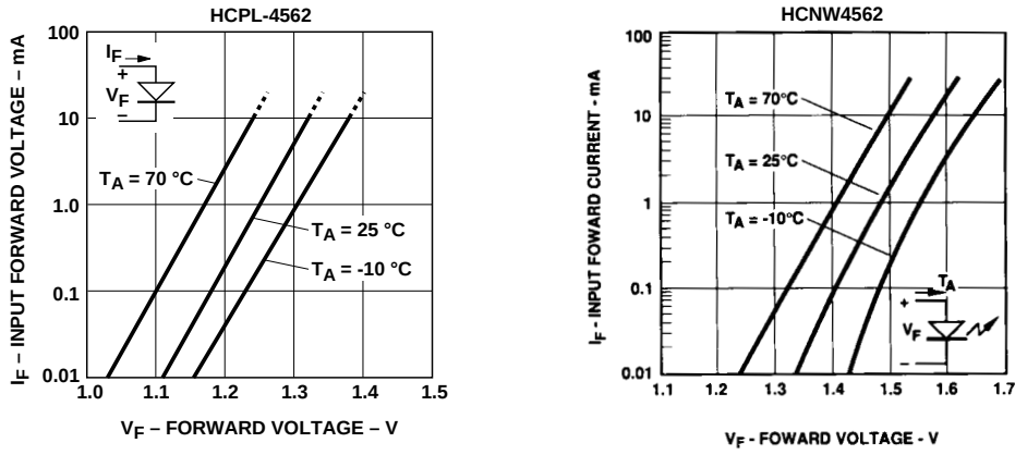
Figure 5. Input Current vs. Forward Voltage.
