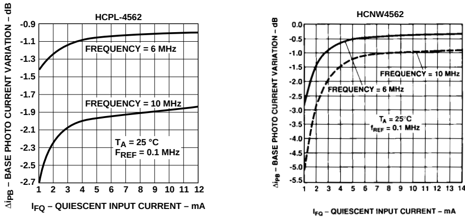
Figure 10. Base Photo Current Variation vs. Bias Conditions.
