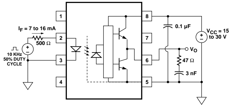
Figure 17. Propagation Delay Test Circuit and Waveforms.
