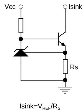
Fig 9. Constant Current Sink
