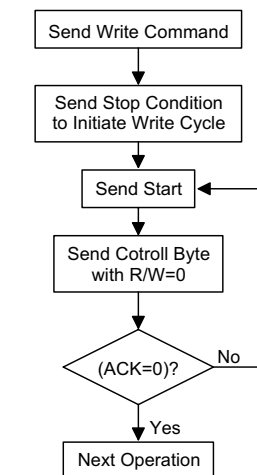
Acknowledge polling flow
