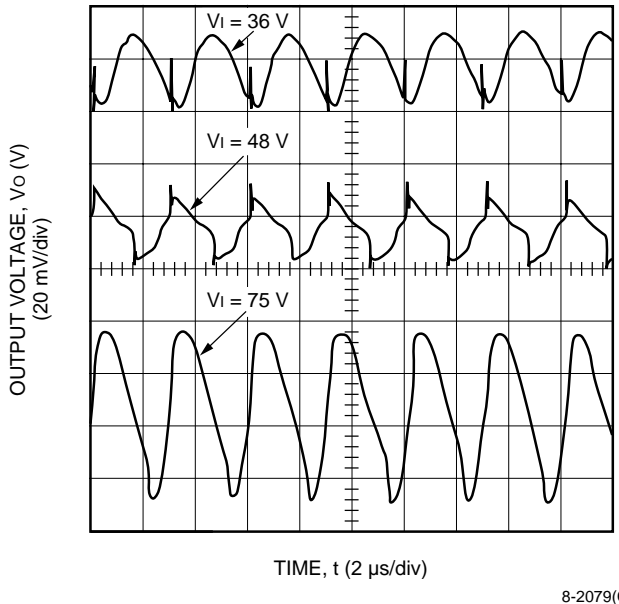
Figure 6. Typical HW100A1 Output Ripple Voltage at Room Temperature and I_o = I_{o,max}
