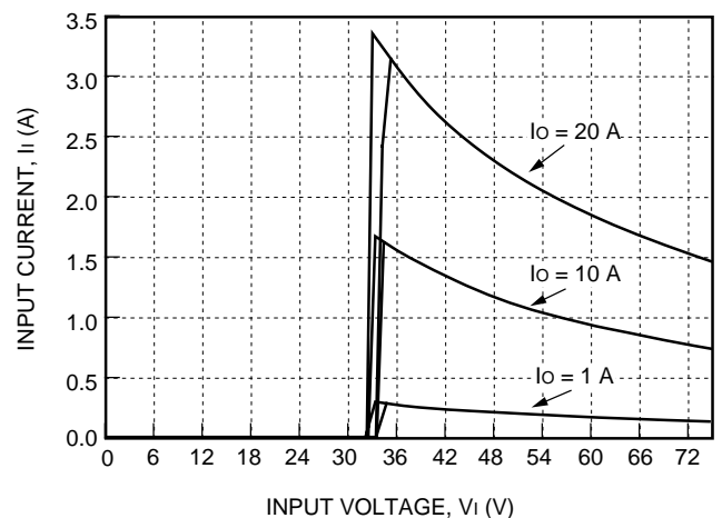
Figure 2. Typical HW100A1 Input Characteristics at Room Temperature
