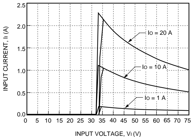
Figure 1. Typical HW100F1 Input Characteristics at Room Temperature
