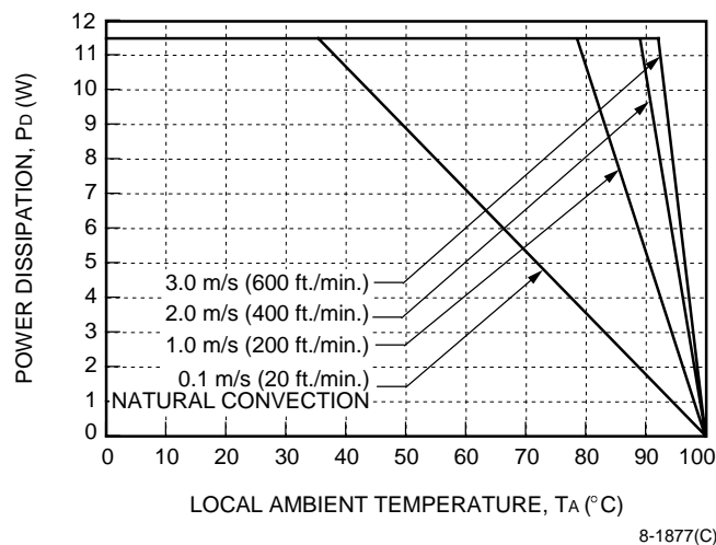
Figure 23. HW100F1 Power Derating vs. Local Ambient Temperature and Air Velocity; Best Orientation
