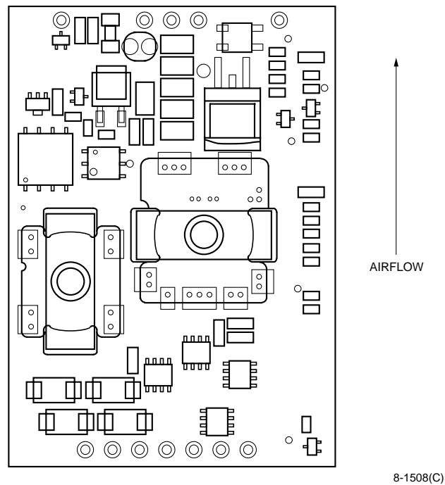
Figure 19. Worst Orientation (Top View)
