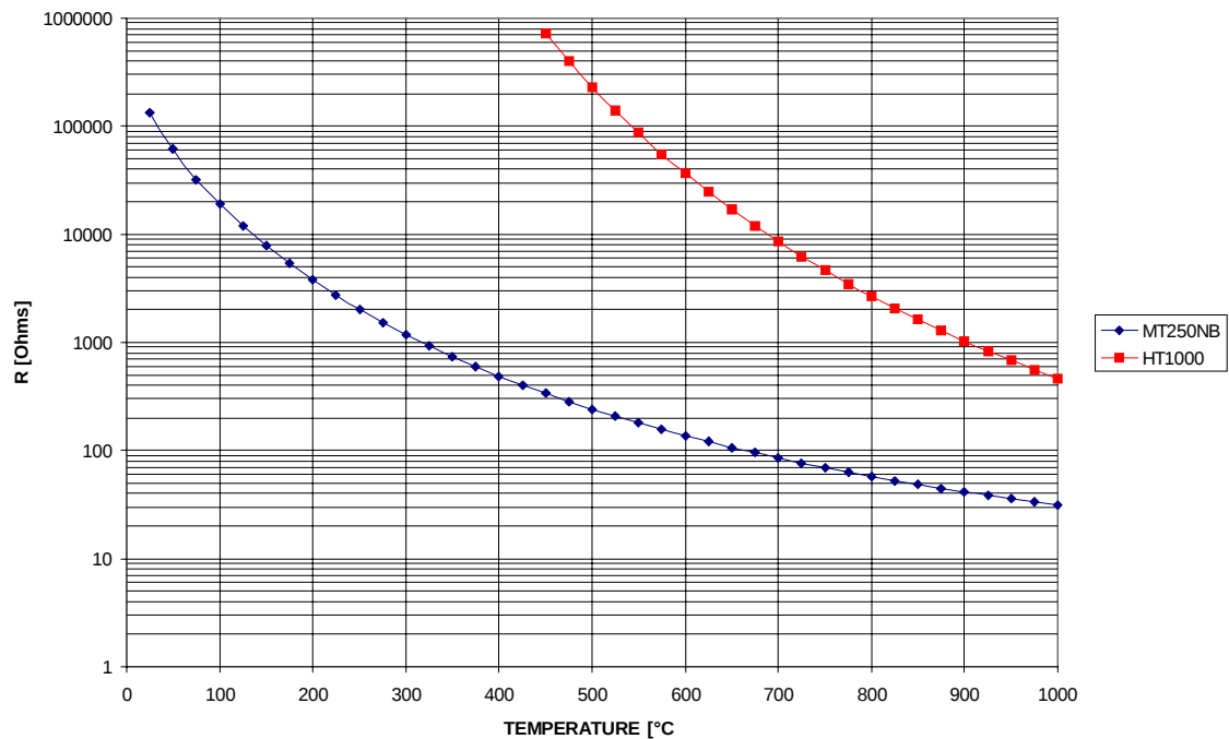
Resistance-temperature Characteristics
