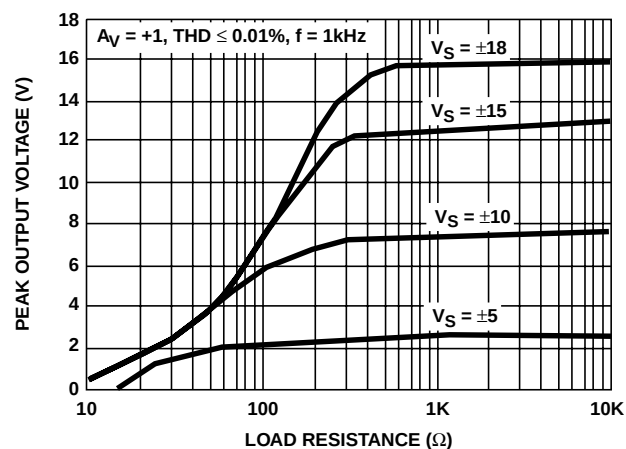
FIGURE 28. OUTPUT VOLTAGE SWING vs LOAD RESISTANCE
