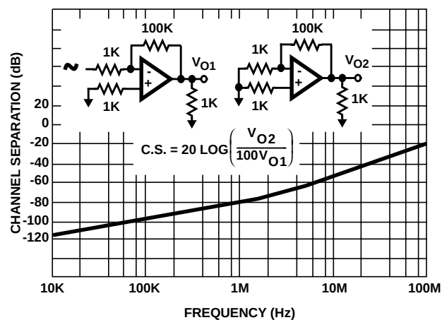
FIGURE 30. CHANNEL SEPARATION vs FREQUENCY
