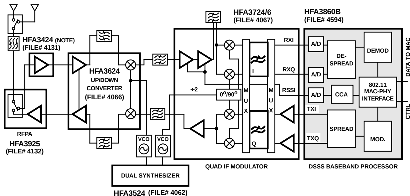
TYPICAL TRANSCEIVER APPLICATION CIRCUIT USING THE HFA3860B
