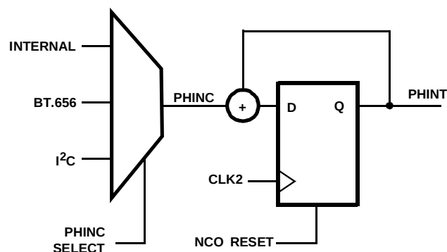
FIGURE 7. COLOR SUBCARRIER GENERATION NCO
