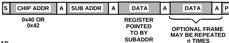
FIGURE 10. I²C SERIAL TIMING FLOW
