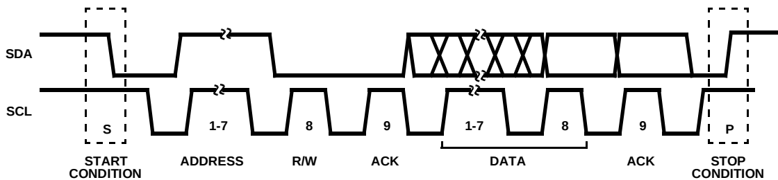
FIGURE 10. I²C SERIAL TIMING FLOW
