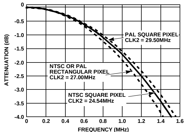
FIGURE 9B. PASS BAND
