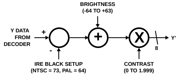
FIGURE 10. LUMINANCE CONTROL SETTINGS PATH
