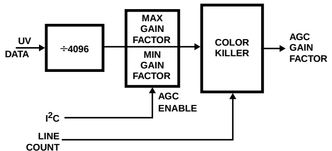
FIGURE 12. LOOP FILTER BLOCK DIAGRAM (HYSTERESIS)
