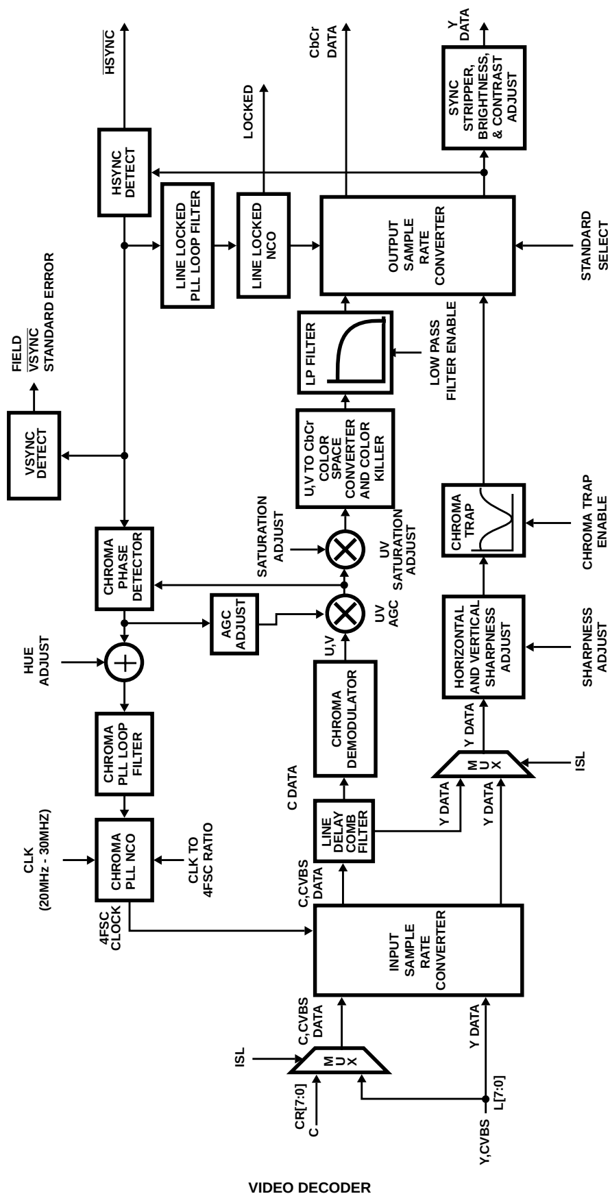
VIDEO DECODER
