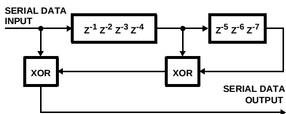
FIGURE 10. SCRAMBLING PROCESS
