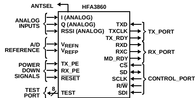
FIGURE 1. EXTERNAL INTERFACE
