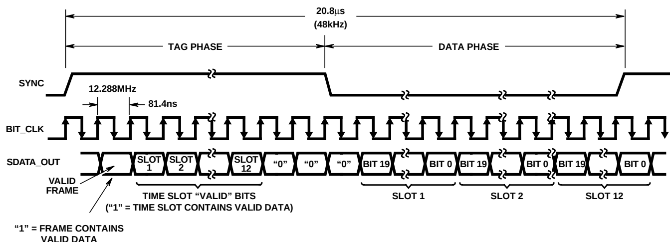
FIGURE 3. AC LINK AUDIO OUTPUT FRAME
