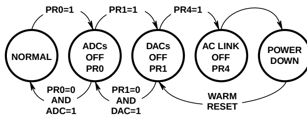
FIGURE 9. HMP9701 POWERDOWN/UP WITH ANALOG ALIVE
