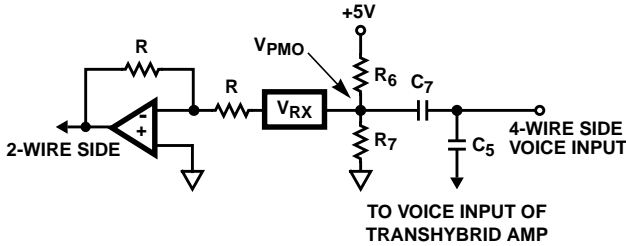
FIGURE 13. PULSE METERING OFFSET GENERATION
