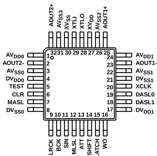
HI2559, CXD2559 (MQFP) TOP VIEW
