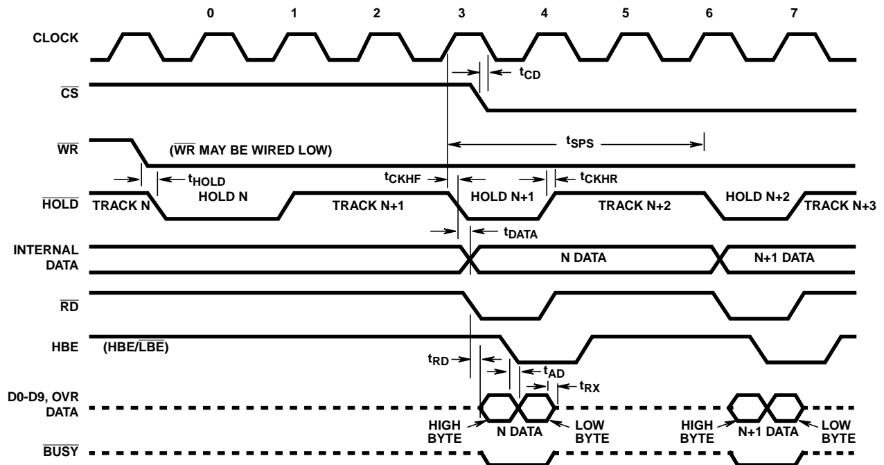
FIGURE 1B. FAST MEMORY MODE (8-BIT DATA BUS)
