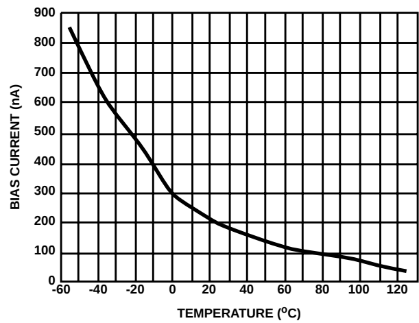
FIGURE 11. BIAS CURRENT vs TEMPERATURE
