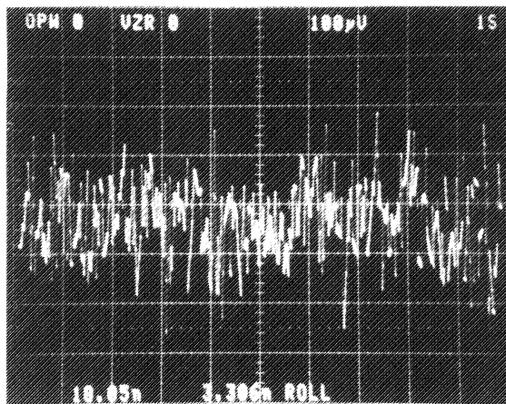
FIGURE 26. INPUT NOISE VOLTAGE 0.1Hz to 10Hz A_V = 25,000 , Noise Voltage = 3.31nV_{RMS} (RTI)
