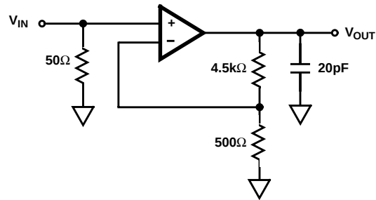
FIGURE 1. LARGE AND SMALL SIGNAL RESPONSE TEST CIRCUIT
