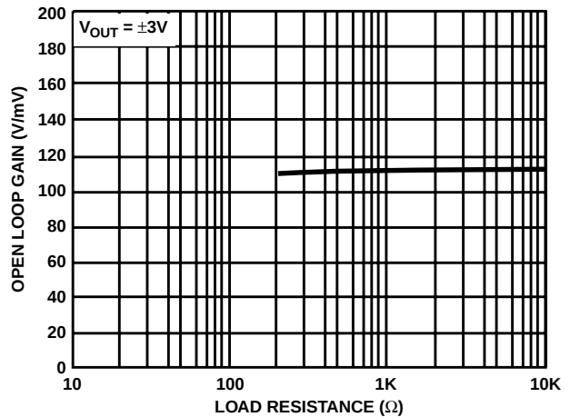
FIGURE 21. OPEN LOOP GAIN vs LOAD RESISTANCE
