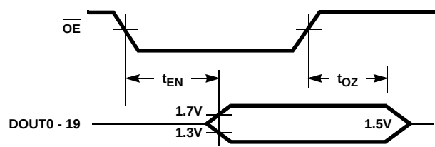
FIGURE 10. THREE-STATE CONTROL
