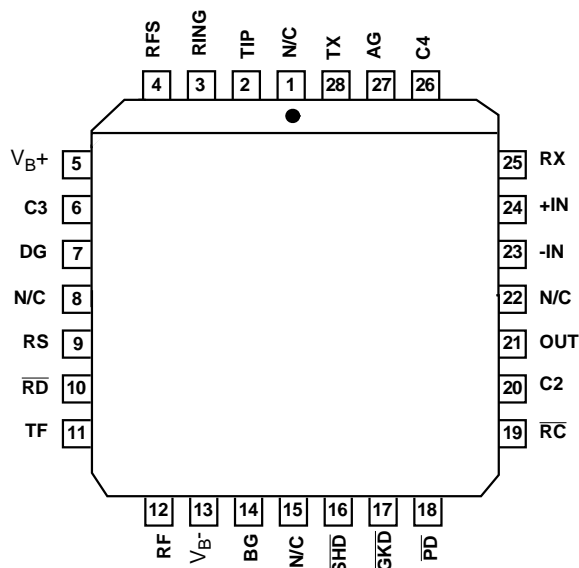
HC-5504DLC (PLCC) TOP VIEW
