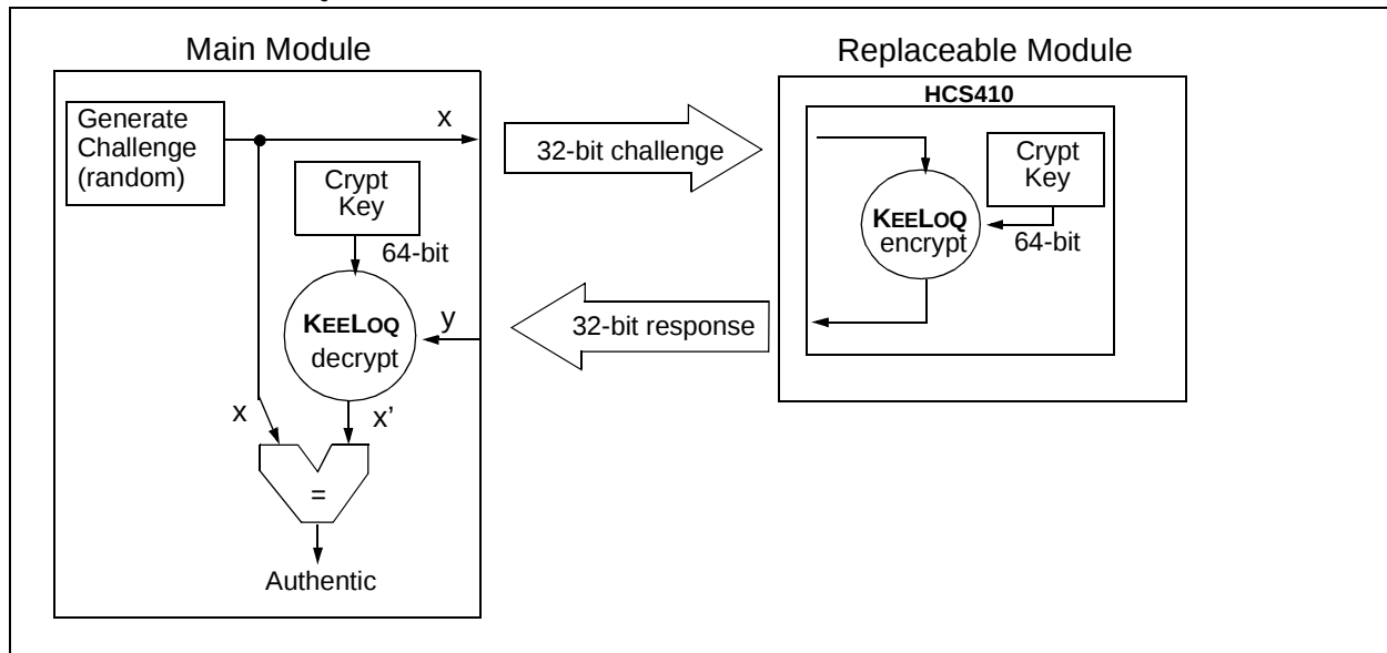
FIGURE 3: KEELOQ - IFF
