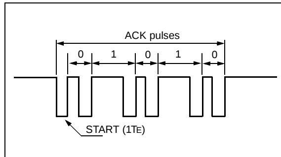
FIGURE 8: ACKNOWLEDGE PULSES
