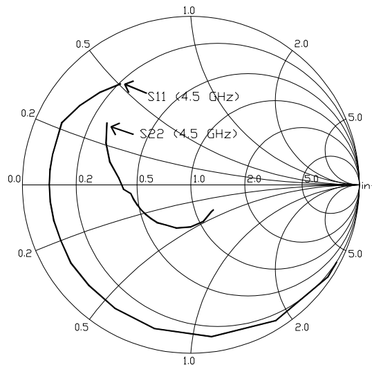
S_{11} & S_{22} vs. Frequency (.05 to 4.5 GHz)
