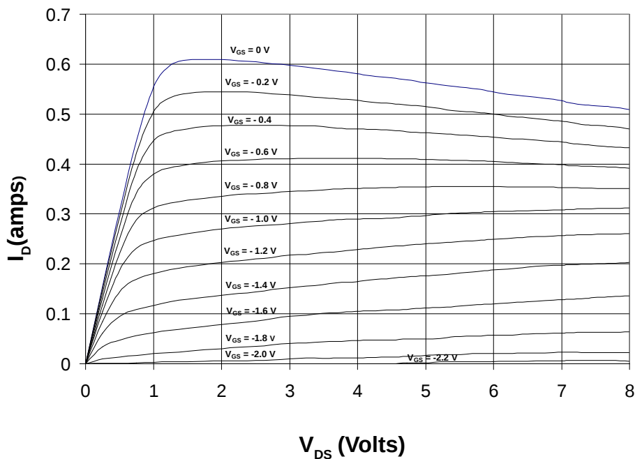
Plot of I_D vs. V_{DS} for V_{GS} = -2.2V to 0V
