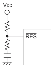
Reset circuit
