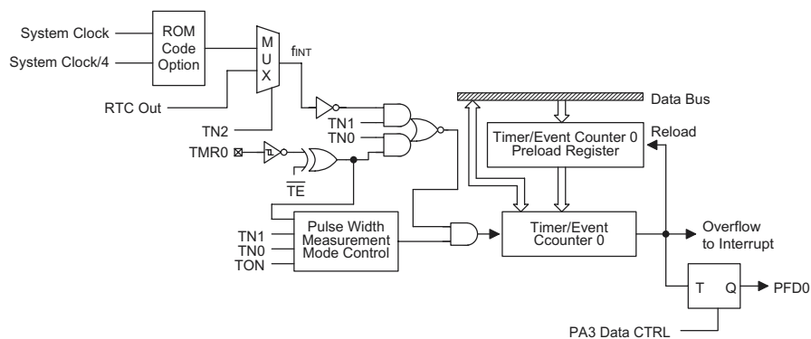
Timer/Event Counter 0
