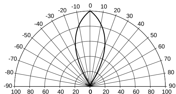
Fig. 4 Radiation Diagram
