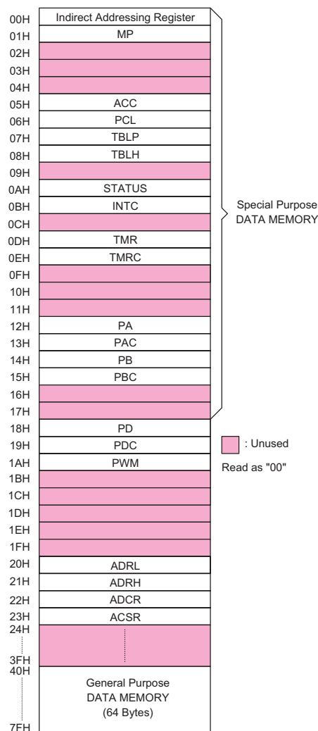
RAM mapping
